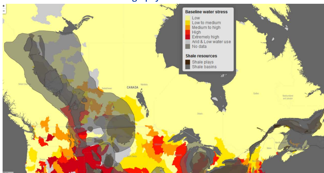
Figure 35 Canada's shale gas plays and baseline water stress
