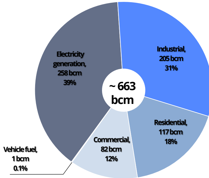
Figure 16 United States natural gas demand by sector, 2013
