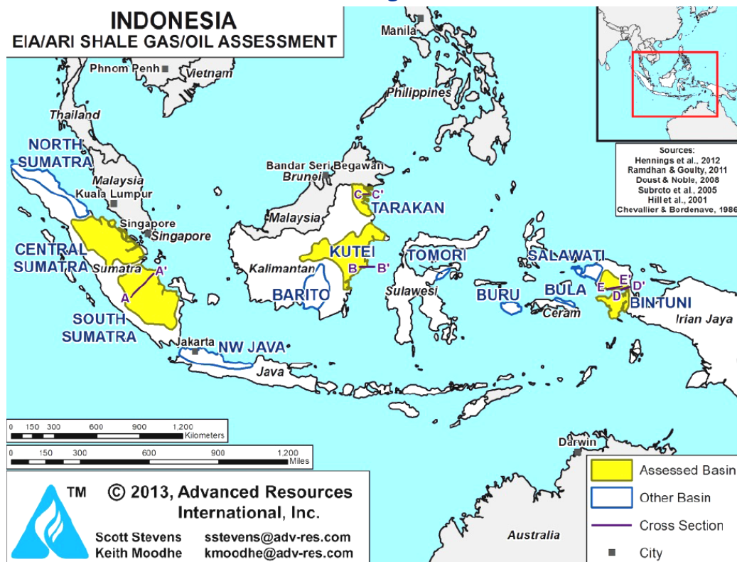
Figure 49 Indonesia’s shale gas resources
