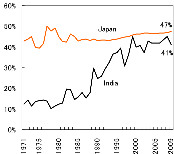
Efficiency of gas-fired power plant
