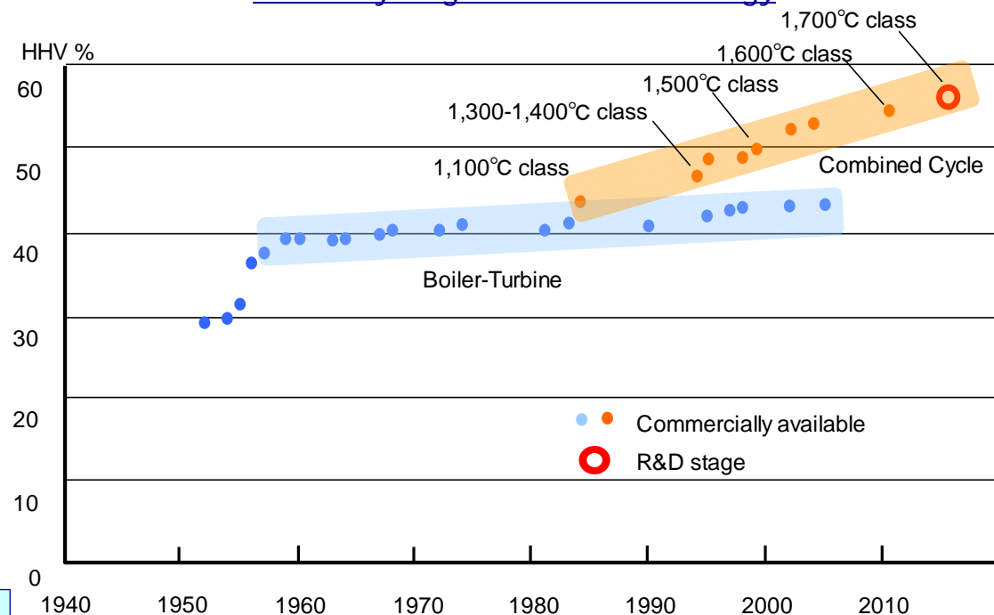
Efficiency of gas turbine technology
