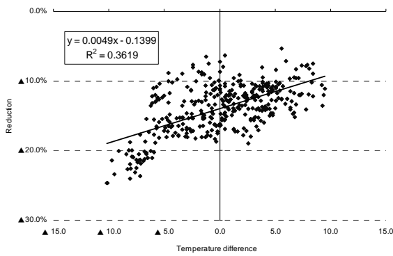
Fig. 3-7 Correlation between Temperature Difference and Reduction (9 a.m.-8 p.m.) (June)
