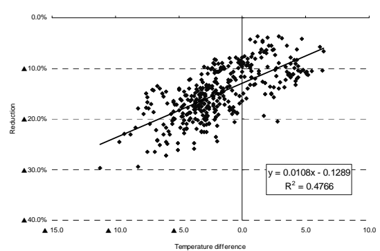
Fig. 3-12 Correlation between Temperature Difference and Reduction (9 p.m.-8 a.m.) (August)
