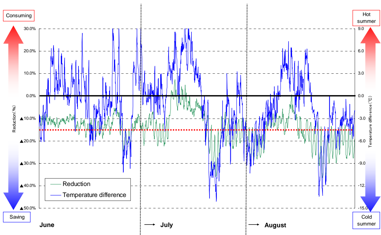
Fig. 2-1 The Temperature Difference and the Reduction of Electricity Demand over the Previous Year (TEPCO) (June-August)
