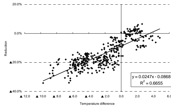
Fig. 3-6 Correlation of between Temperature Difference and Reduction (9 p.m.-8 a.m.) (August)
