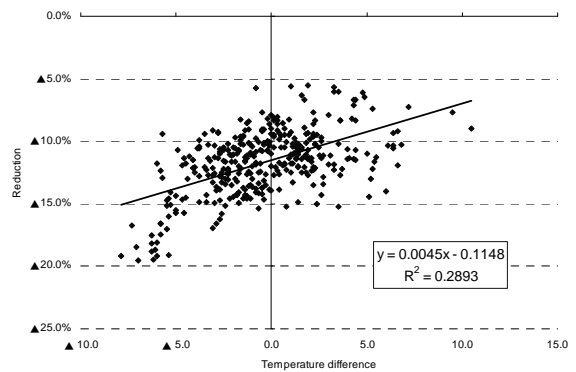
Fig. 3-8 Correlation between Temperature Difference and Reduction (9 p.m.-8 a.m.) (June)
