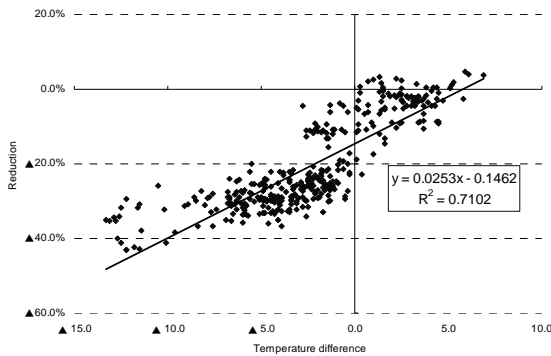
Fig. 3-5 Correlation of between Temperature Difference and Reduction (9 a.m.-8 p.m.) (August)
