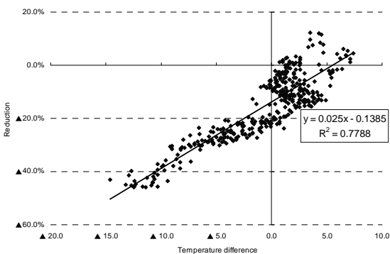
Fig. 3-3 Correlation of between Temperature Difference and Reduction (9 a.m.-8 p.m.) (July)
