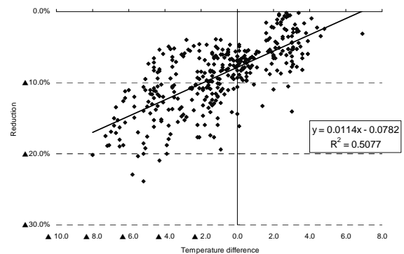
Fig. 3-2 Correlation of between Temperature Difference and Reduction (9 p.m.-8 a.m.) (June)
