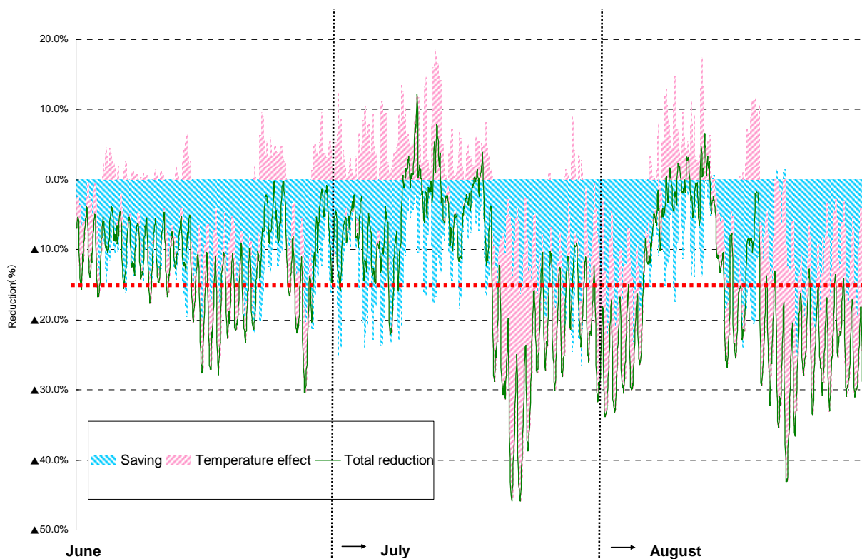
Fig. 4-1 The Breakdown of Factors (TEPCO) (June-August)
