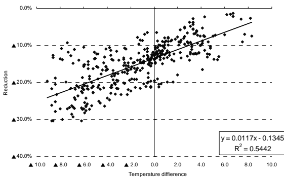
Fig. 3-1 Correlation of between Temperature Difference and Reduction (9 a.m.-8 p.m.) (June)
