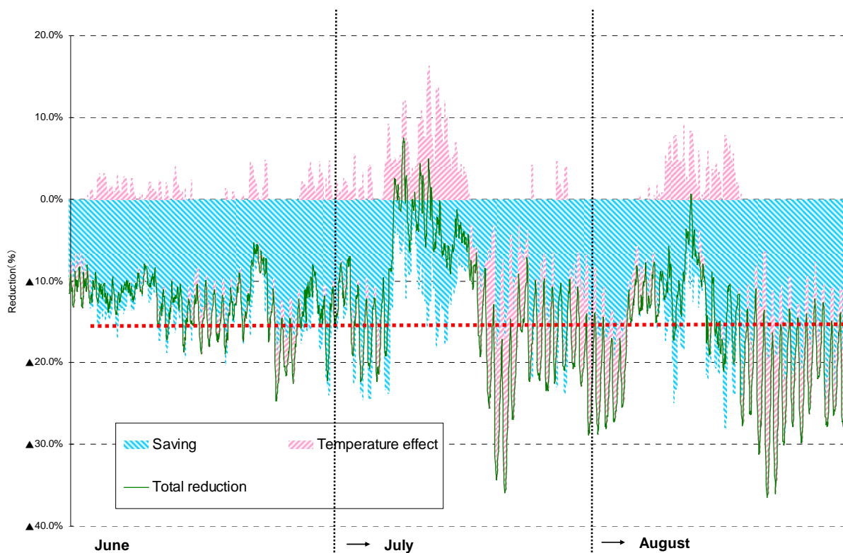
Fig. 4-2 The Breakdown of Factors (Tohoku Electric) (June-August)
