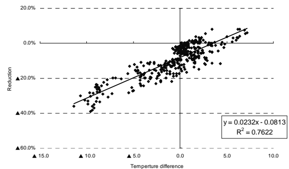
Fig. 3-4 Correlation of between Temperature Difference and Reduction (9 p.m.-8 a.m.) (July)
