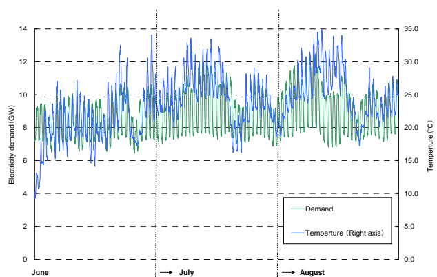
Fig. 1-2 Tohoku Electric Power Company
