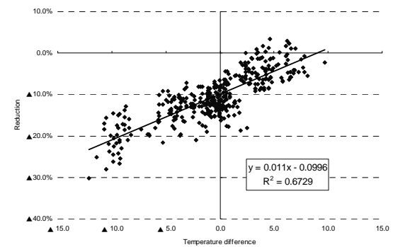
Fig. 3-10 Correlation between Temperature Difference and Reduction (9 p.m.-8 a.m.) (July)
