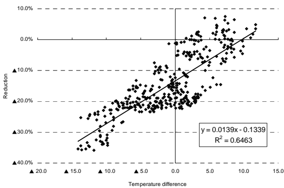
Fig. 3-11 Correlation between Temperature Difference and Reduction (9 a.m.-8 p.m.) (August)
