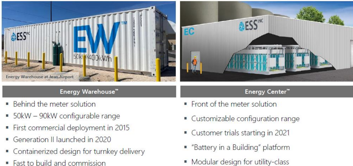
Fig. 10 ESS' iron flow battery product lineup
