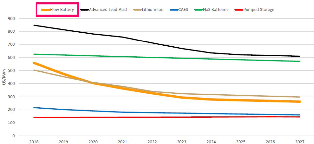
Fig. 15 Projected energy storage technology equipment costs (2018-2027)
