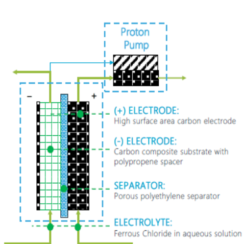
Fig. 6 Principle of operation for IFBs
