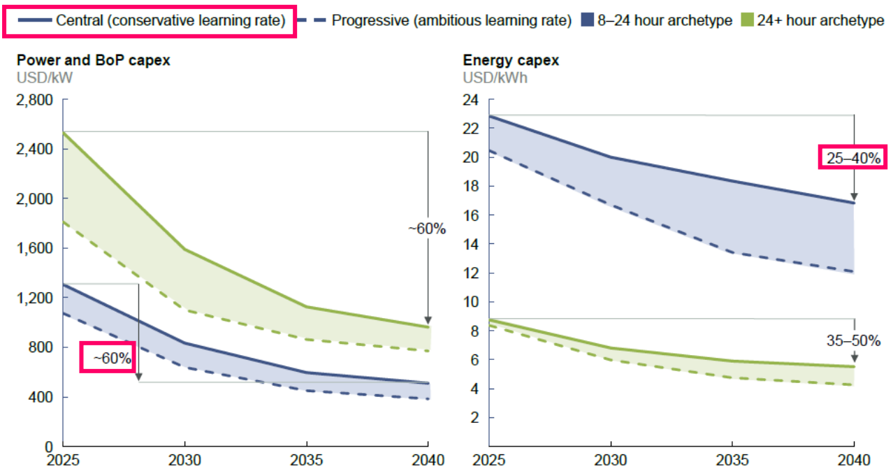
Fig. 2 Outlook on long-duration energy storage technology costs (2025-2040)
