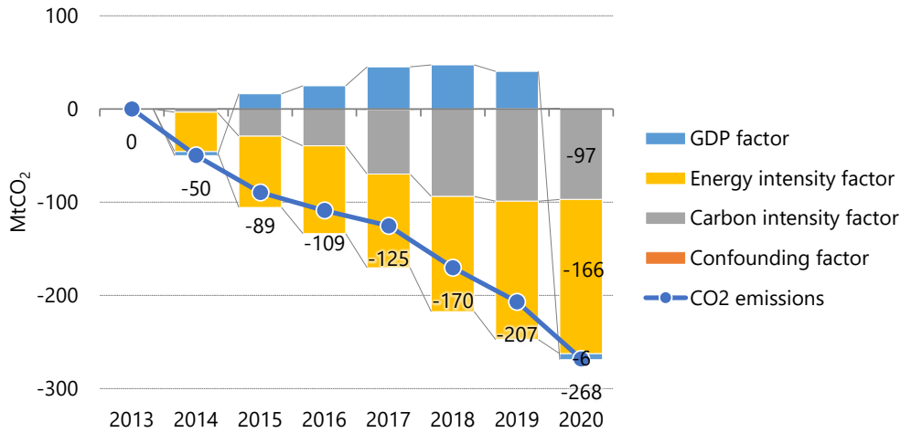
Fig. 2 Decomposition analysis of CO 2 emissions
