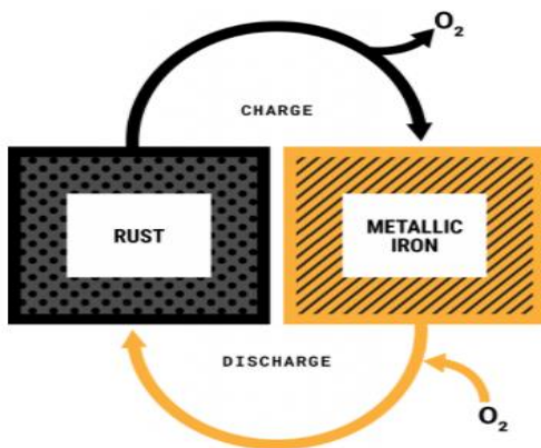
Fig. 11 Principle of operation of iron-air batteries
