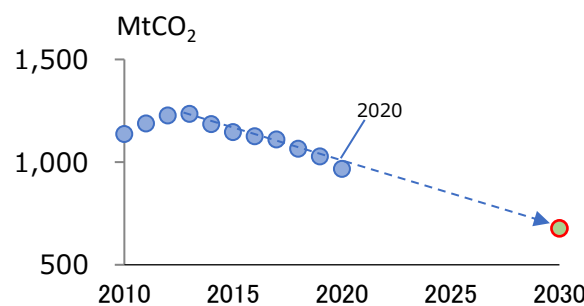
Fig. 1 CO 2 emissions and the target
